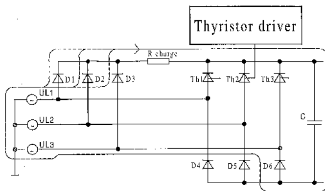
Fig. 3 Charge circuit
